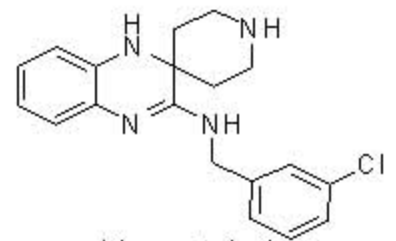
Liproxstain-1 C 19 H 21 ClN 4 DMSO-d 6
